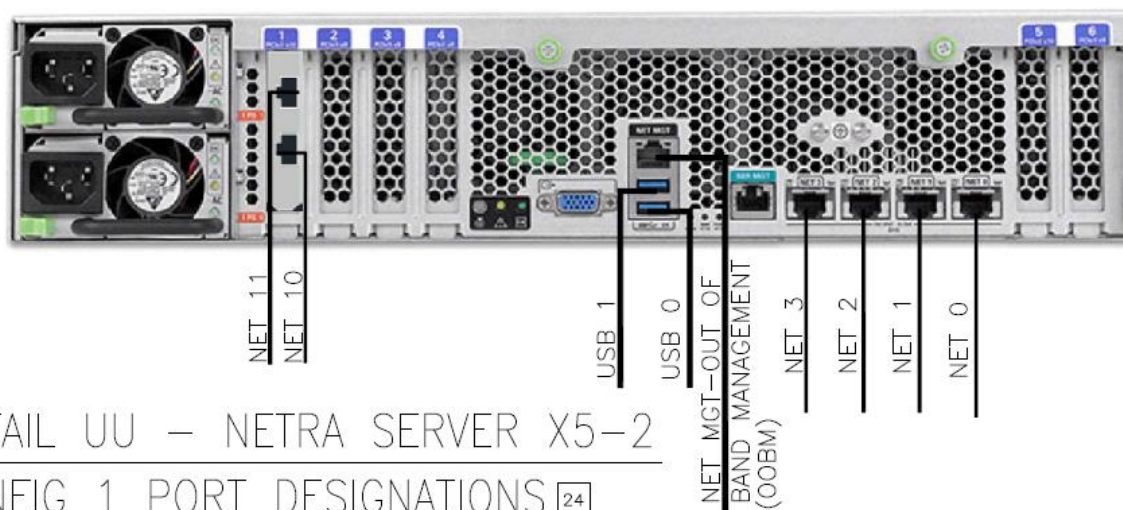
Figure 11: Netra X5-2 Config 1 Port Designations
