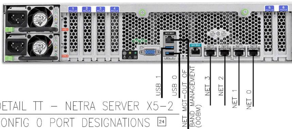
Figure 10: Netra X5-2 Config 0 Port Designations
